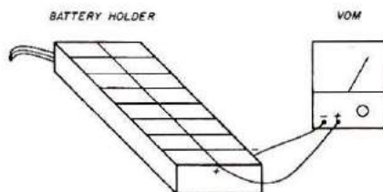
Fig. 1. Battery voltage should be checked under normal load conditions. Measure the voltage across each cell while the receiver, or other device, is turned on.
